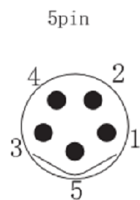
Pin assignment front view/针位分布前视图
