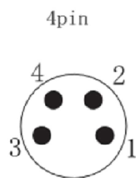
Pin assignment front view/针位分布前视图
